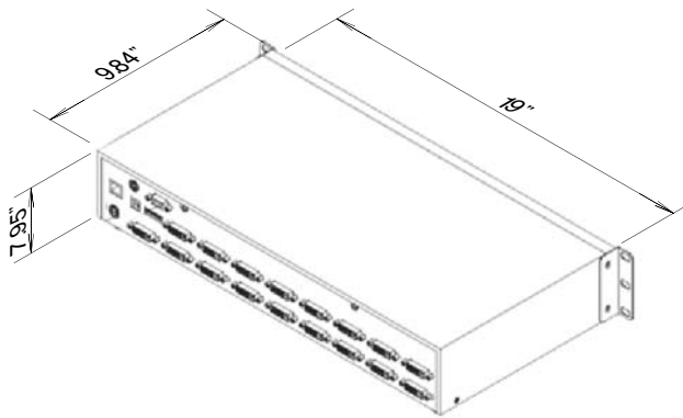
VX-DVI-8000 (Back View)
